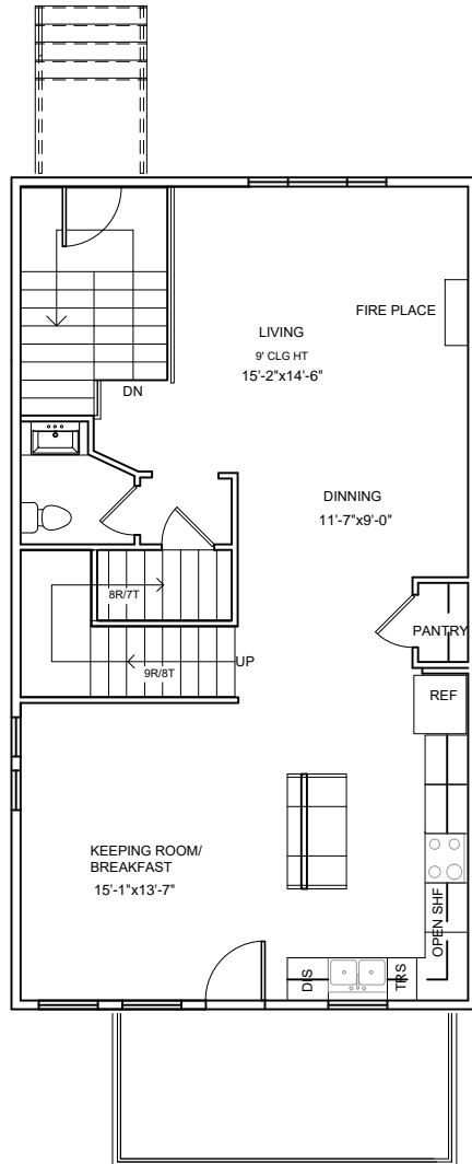
BUILDING 2 TYPE B: SECOND FLOOR PLAN
