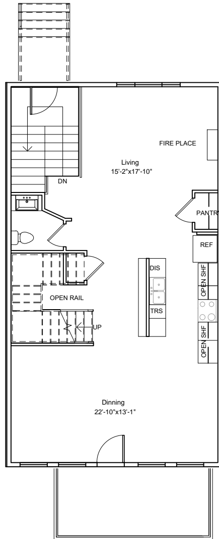
BUILDING 2 TYPE A: SECOND FLOOR PLAN
